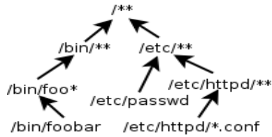
Figure 3: An example FCGlob tree.
